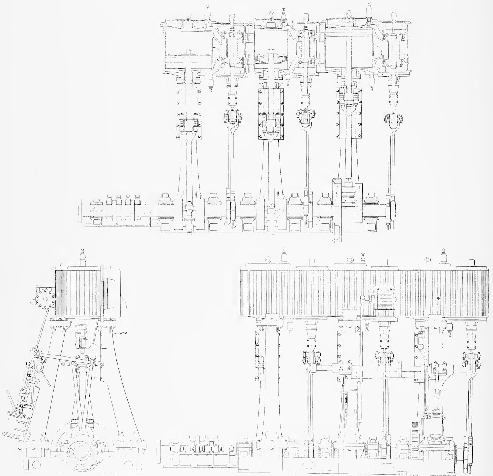
THREE CYLINDER COMPOUND ENGINES OF THE FERRY STEAMER PLEASURE.— Built by F. W. Wheeler & Co., West Bay City, Mich.
